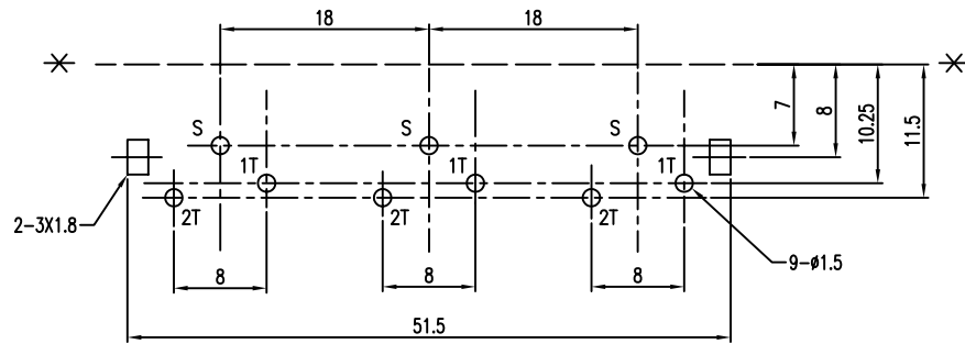
T:1.6 Dimensions of PC board holes Tolerance : ±0.1(Printed-bottom view)
