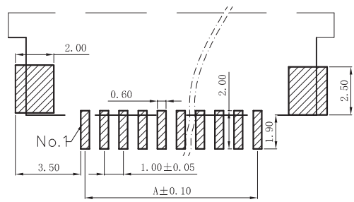
PCS Layout
