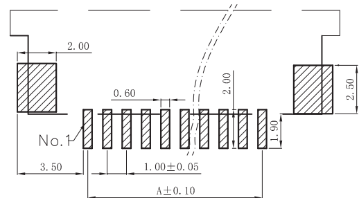
PCS Layout
