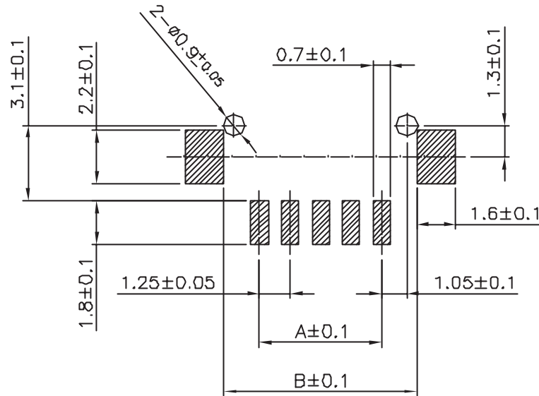
Recommend PCB Layout
