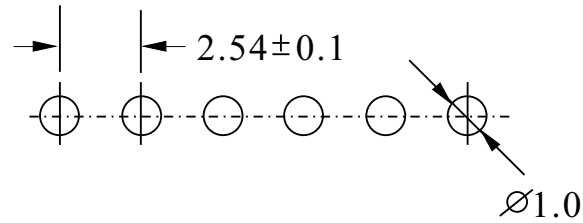
Recommmand PCB Layout
