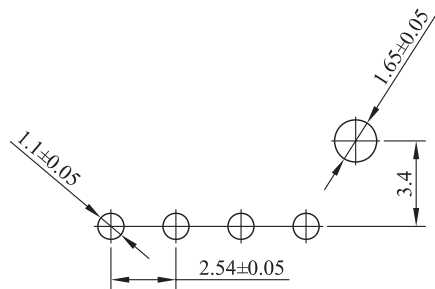
RECOMMENDED P.C. BOARD HOLE DIMM.
