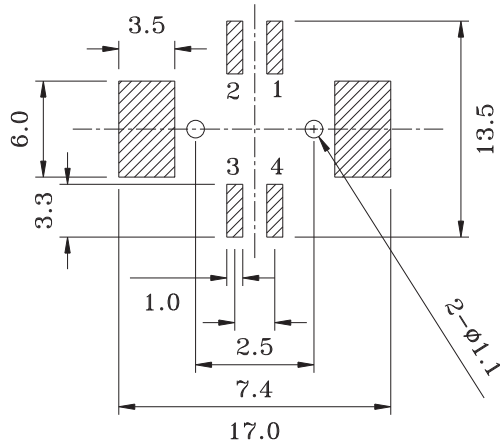
(COMPONENT SIDE) PCB LAYOUT
