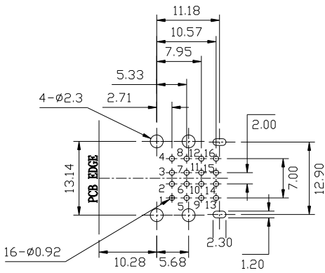
BOTTOM VIEW RECOMMENDED PCB LAYOUT A
