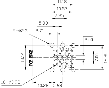
BOTTOM VIEW RECOMMENDED PCB LAYOUT B
