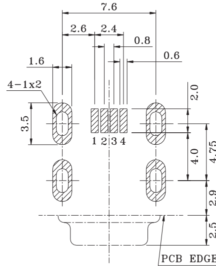
COMPONENT SIDE PCB LAYOUT
