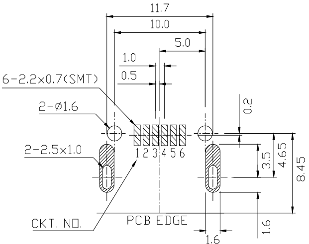
(COMPONENT SIDE) PCB LAYOUT
