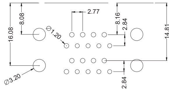
RECOMMEND P.C.B. LAYOUT BOTTOM VIEW
