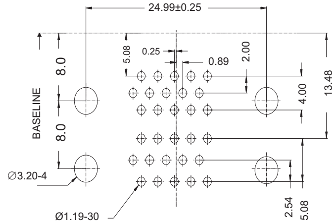
RECOMMEND P.C.B. LAYOUT BOTTOM VIEW
