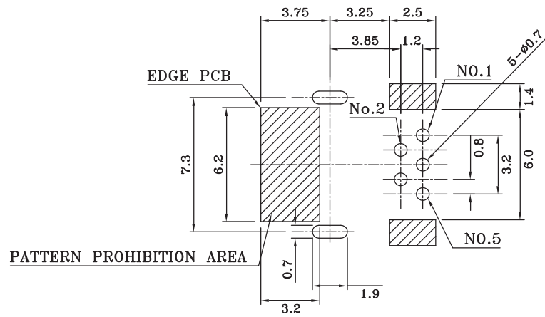
RECOMMENDED PCB PATTERN LAYOUT (PCB THICKNESS:0.8±0.1)
