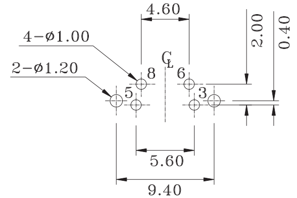
COMPONENT SIDE (PCB LAYOUT)
