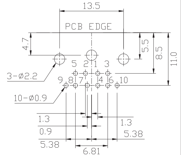
P.C.B. RECOMMEND LAYOUT BOTTOM VIEW
