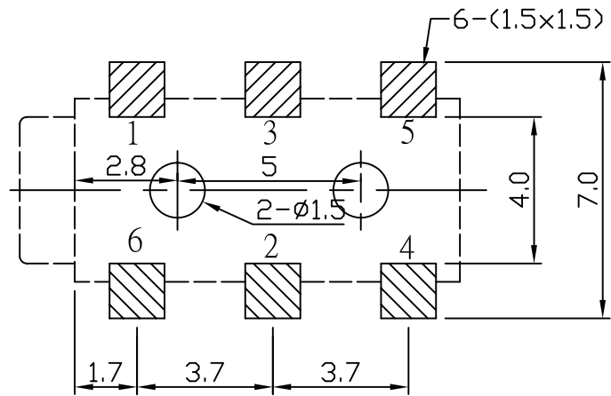
T:1.6 Dimensions of PC board holes Tolerance : \pm 0.1 (Printed-top view)
