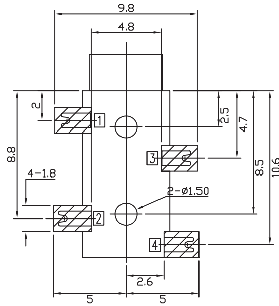
Recommended PCB Layout Tolerance: ±0.1(Printed-side view)
