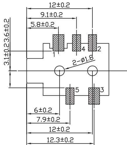
T:1.6 Dimensions of PC board holes Tolerance : ±0.1(Printed-top view)
