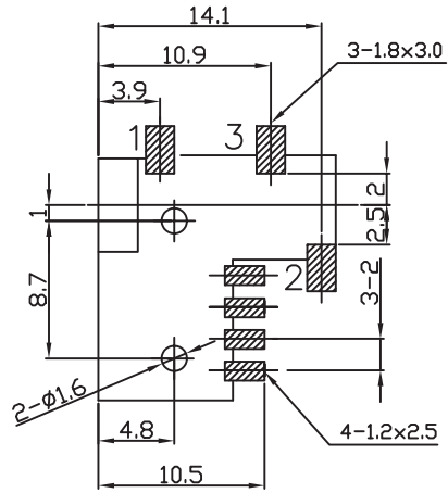
T:1.6 Dimensions of PC board holes Tolerance : \pm 0.1 (Printed-top view)
