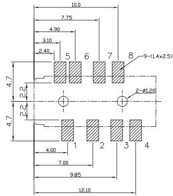
T:1.6 Dimensions of PC board holes Tolerance : ±0.1(Printed-top view)
